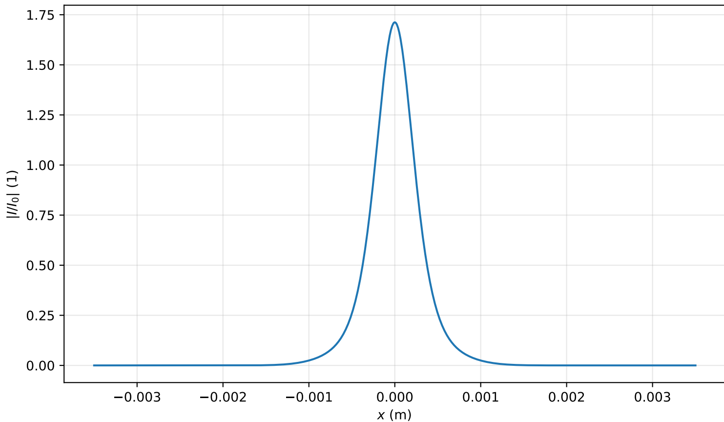
Intensity profile I(x, y = 0, z = 1.274m)/I_0 , P_{in}=1.0P_{cr} , artificial time
